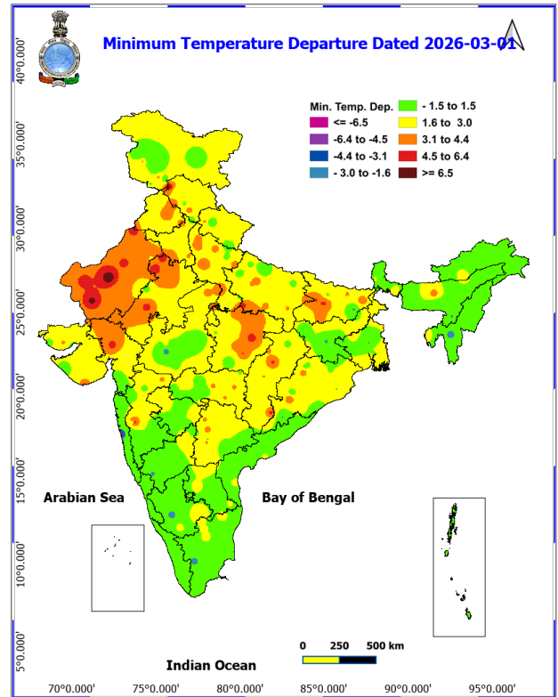
Fig. 4: Departure of Minimum Temp. Dated 2026-03-01
