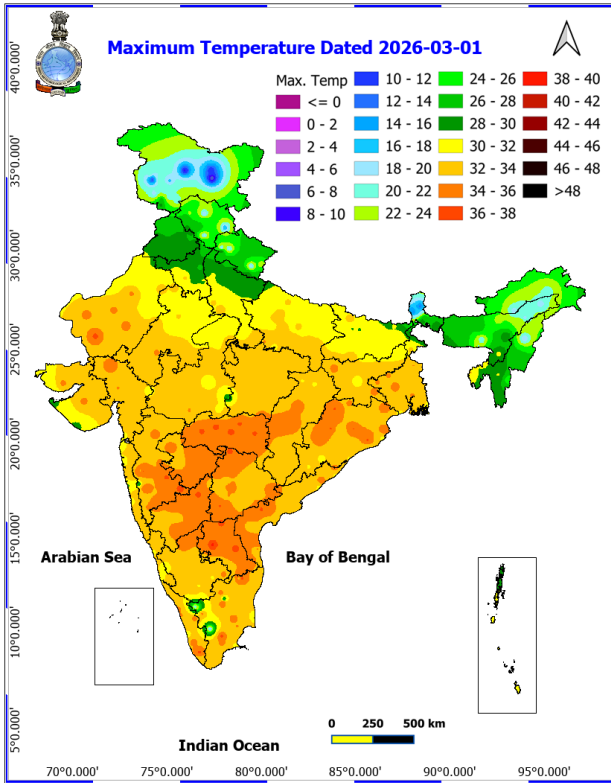
Fig. 1: Maximum Temperatures Dated 2026-03-01
