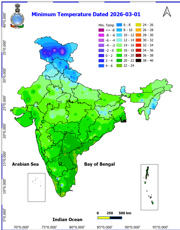
Fig. 3: Minimum Temperatures Dated 2026-03-01
