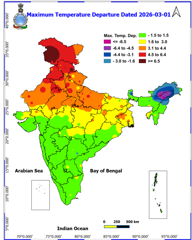
Fig. 2: Departure of Maximum Temp. Dated 2026-03-01
