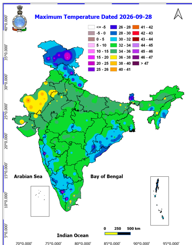
Fig. 1: Maximum Temperatures Dated 2026-09-28
