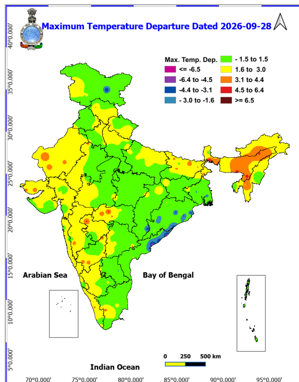
Fig. 2: Departure of Maximum Temp. Dated 2026-09-28
