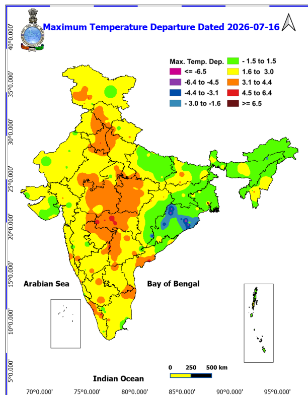
Fig. 2: Departure of Maximum Temp. Dated 2026-07-16
