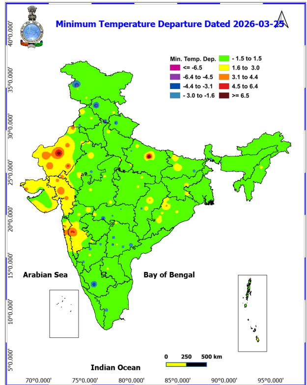
Fig. 4: Departure of Minimum Temp. Dated 2026-03-25
