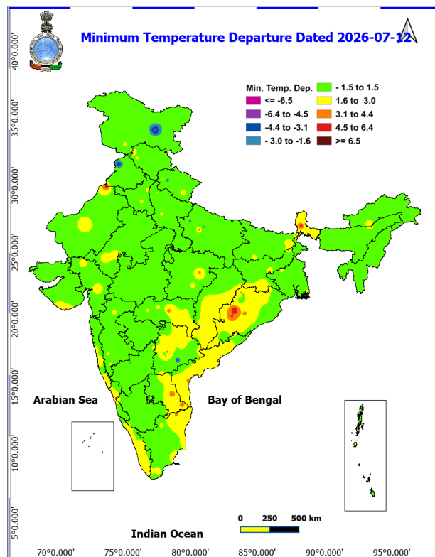
Fig. 4: Departure of Minimum Temp. Dated 2026-07-12
