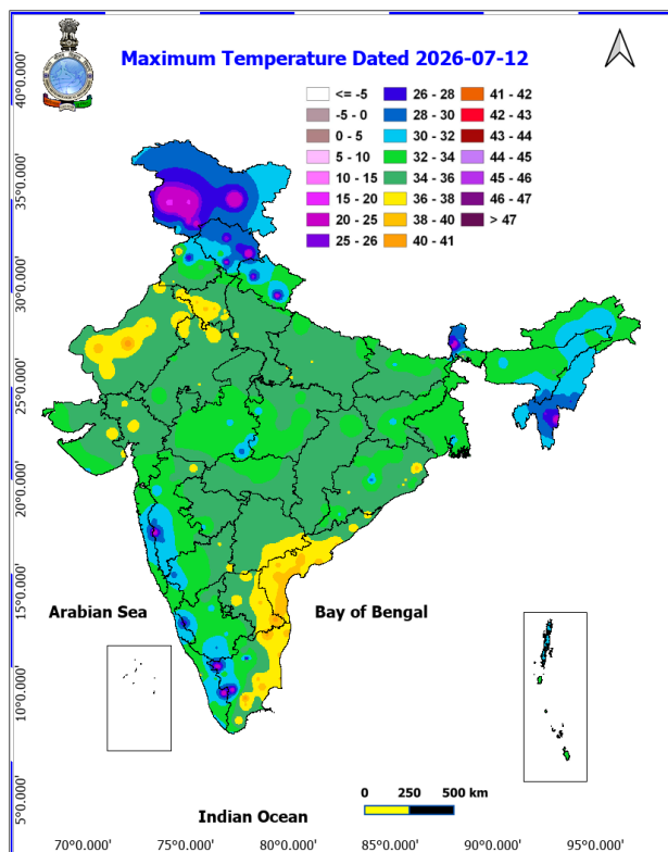
Fig. 1: Maximum Temperatures Dated 2026-07-12
