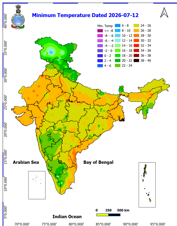
Fig. 3: Minimum Temperatures Dated 2026-07-12
