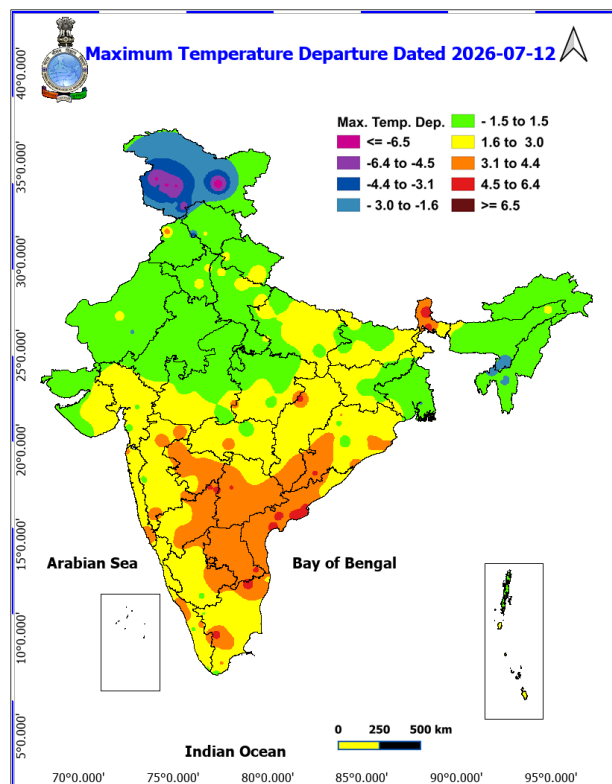
Fig. 2: Departure of Maximum Temp. Dated 2026-07-12
